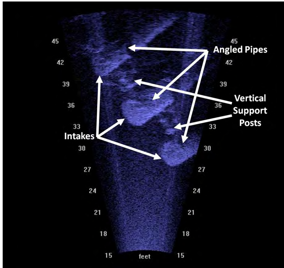
Appendix Figure 45. DIDSON TM still image of the angled pipe intakes at the Portuguese Bend pump station (looking upstream). Woody debris at the downstream end of the pipe intakes is not shown. Image taken on July 3, 2008.
