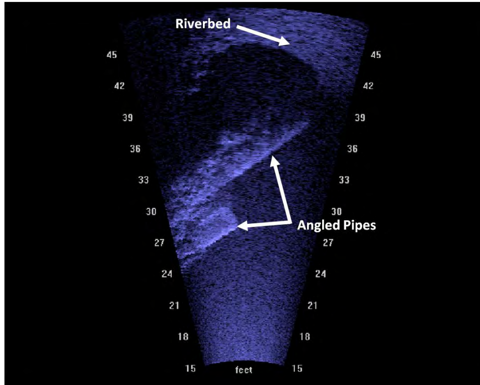
Appendix Figure 73. DIDSON TM still image of the angled pipe intakes at the Cranmore pump station (looking in a downstream direction). Image taken on July 22, 2008.
