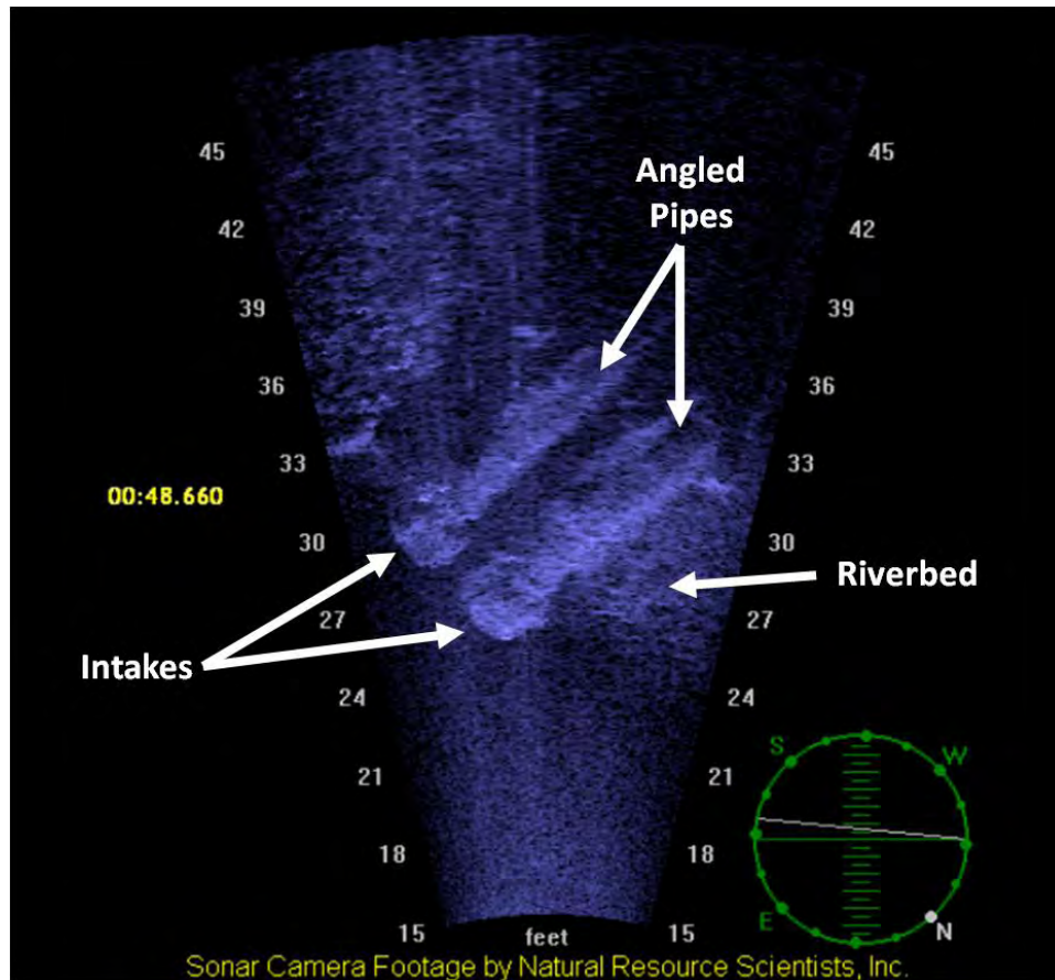
Appendix Figure 3. DIDSON™ still image of two angled pipe intakes at the Sycamore pump station (looking in a downstream direction). Image taken on August 21, 2008.
