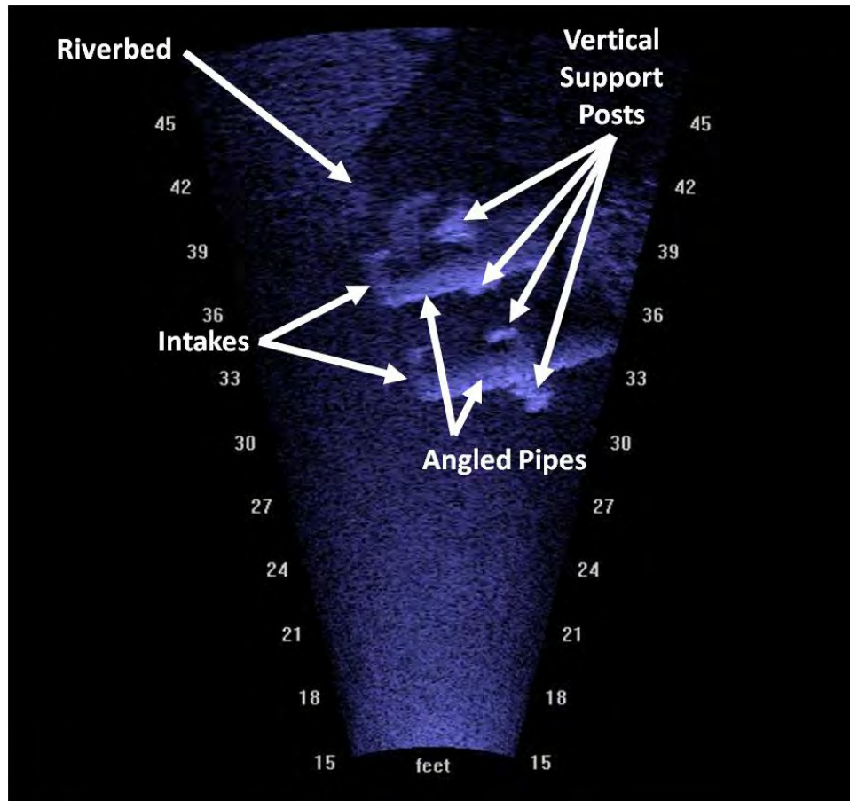
Appendix Figure 31. DIDSON TM still image of the two angled pipe intakes at the Oji pump station (looking upstream). Image taken on July 17, 2008.
