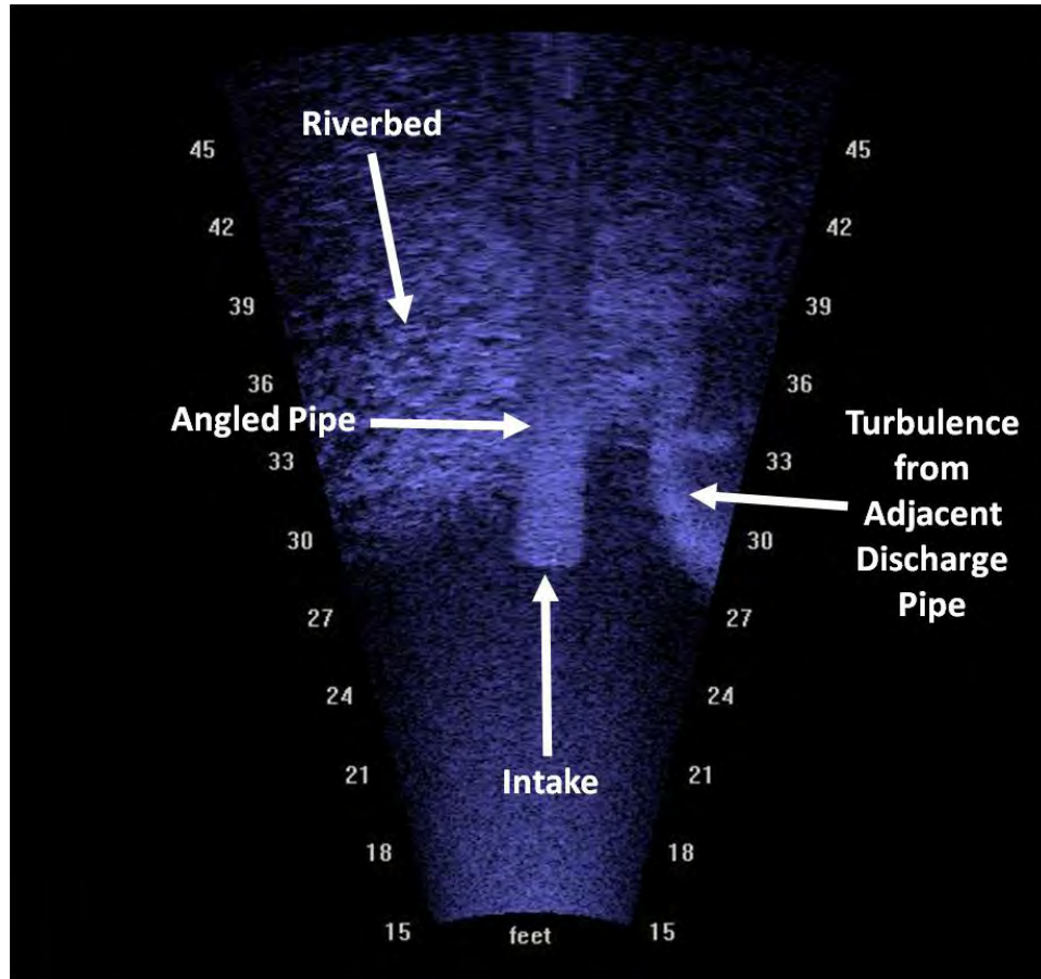
Appendix Figure 38. DIDSON TM still image of the angled pipe intake at the Windswept pump station (looking toward the levee). Image taken on July 17, 2008.
