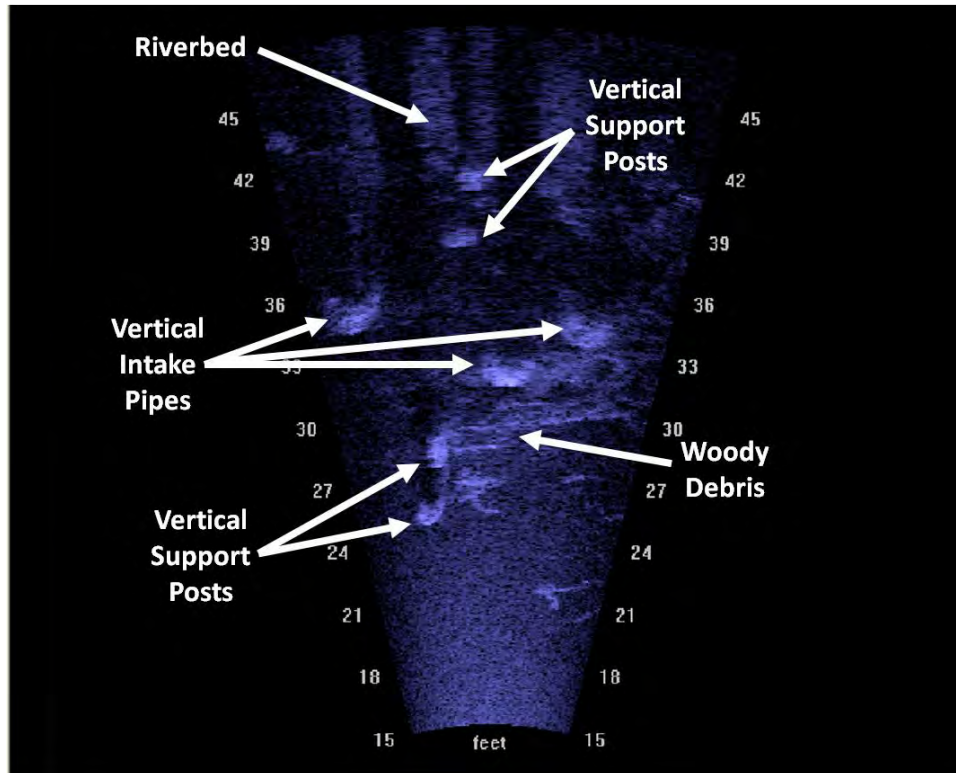
Appendix Figure 59. DIDSON TM still image of the vertical pipe intakes at the Townsite pump station (looking toward the river bank). Image taken on July 8, 2008.
