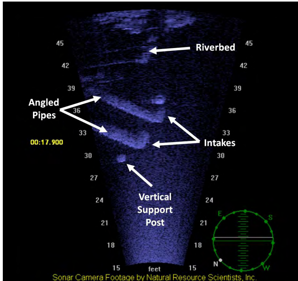
Appendix Figure 10. DIDSON TM still image of two angled pipe intakes at the River Garden Farms No. 2 pump station (looking in an upstream direction). Image taken on July 16, 2008.
