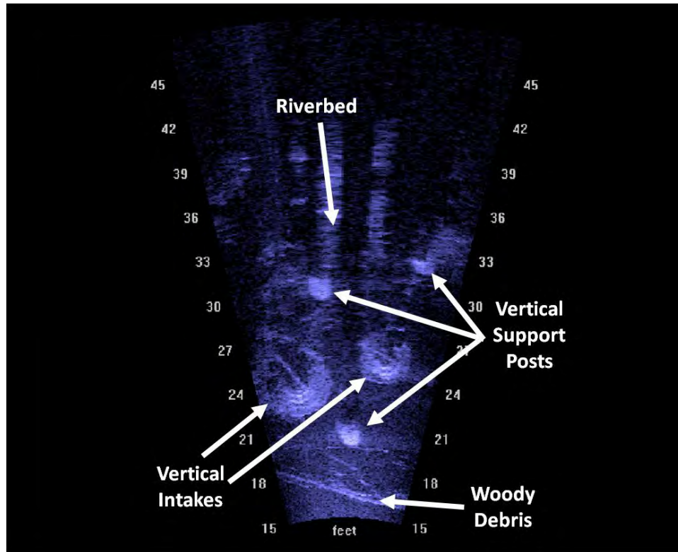
Appendix Figure 66. DIDSON TM still image of the vertical pipe intakes at the Tisdale pump station (looking toward the river bank). Image taken on August 5, 2008.
